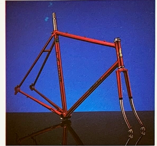
Reynolds 531c. main tubes, 27" H.P. clearance Gents 21½" 23" 24½" Ladies 19½" 21" 23"
