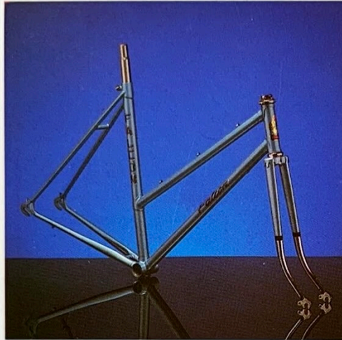
Hi-ten tubing, 27" H.P. clearance Gents 19½" 21½" 23" 24½" Ladies 19½" 21"
