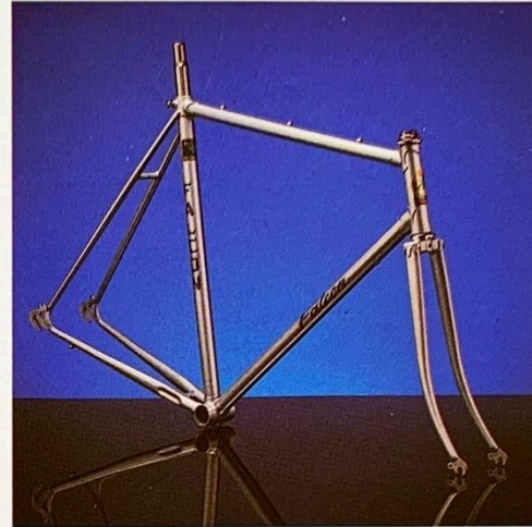
Reynolds 501 main tubes, 27" H.P. clearance Gents 21½" 23" 24½" Ladies 19½" 21"
